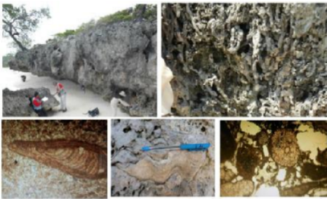
Figure 7 Ourcrop of back reef facies along the west coast (A) with abundant branching coral (B) and small amount of red algae in thin section (C) rare Tridacna sp (D) and Calcarina spin thin section (E).
